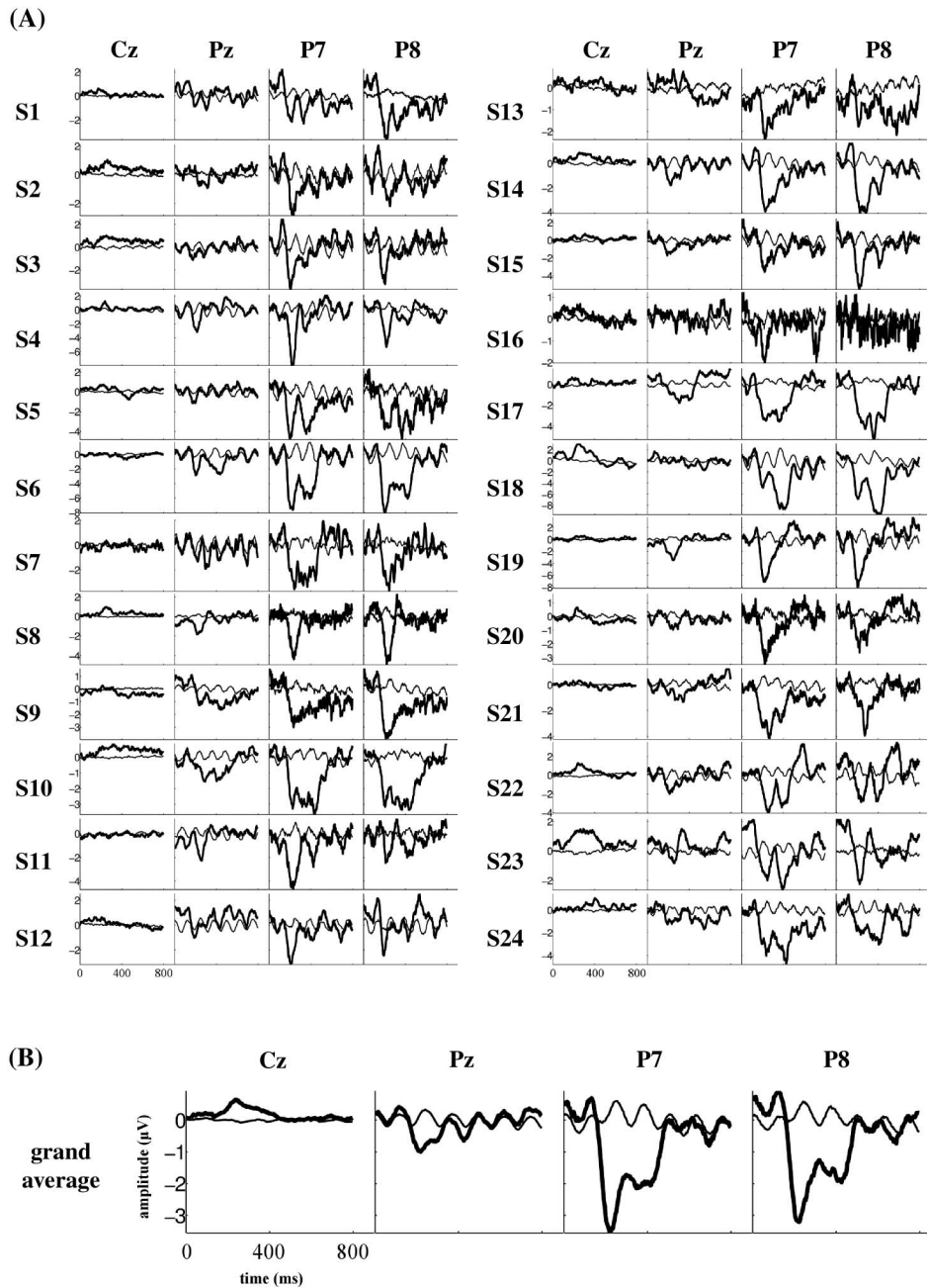
FIG. 6. (A) ERP waveforms elicited from each participant by both target (thick line) and nontarget (thin line) intensifications at four electrode locations: Cz, Pz, P7, and P8. (Amplitude units are \mu\text{V} ; time units are ms.) (B) Grand-averaged ERP waveform elicited by both target (thick line) and nontarget (thin line) intensifications for all 24 participants at four electrode locations: Cz, Pz, P7, and P8.
